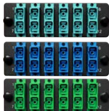
HDA SC Adapter Plate FPP-AD-Sx2-06-A
