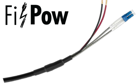
Designed for long distance/high power. FiPOW Indoor/Outdoor Hybrid Cable (Fiber with copper conductors) Available 1-24 Fiber, 2-16 conductors, 12 or 16 AWG
