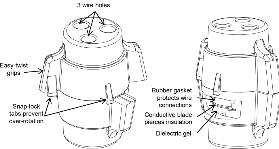
Closed, locked position. Twist clock-wise to close.
